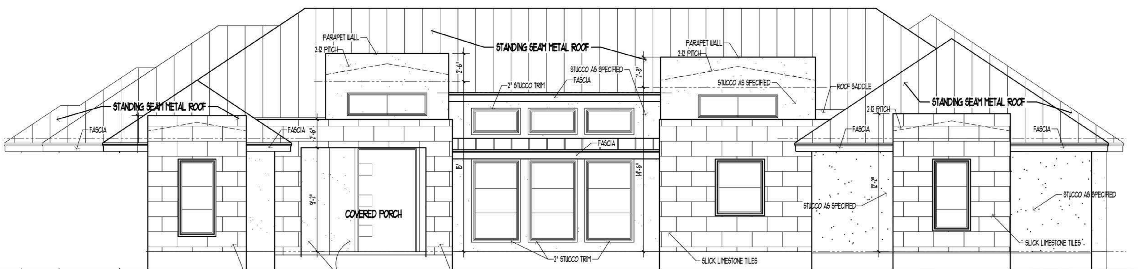
600 FRONT ELEVATION
